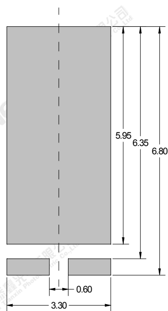
recommended stencil pattern
