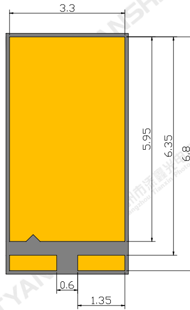
Bottom view
