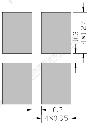
Recommended solder pad
