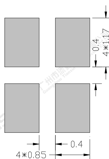
recommended stencil pattern
