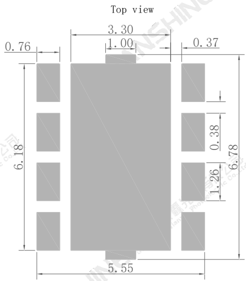
Recommended solder pad
