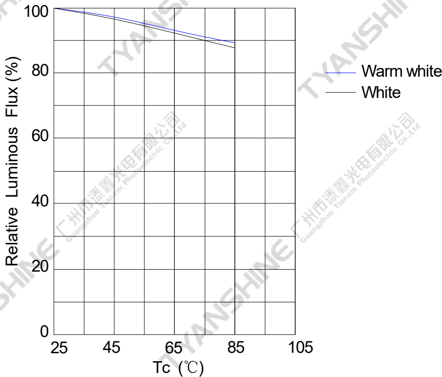
Temperature VS. Relative Luminous Flux (IF=500mA)
