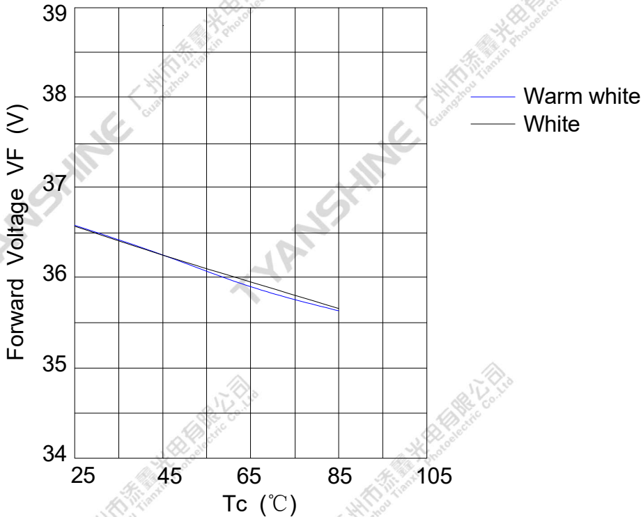
Temperature VS. Forward Voltage (IF=500mA)
