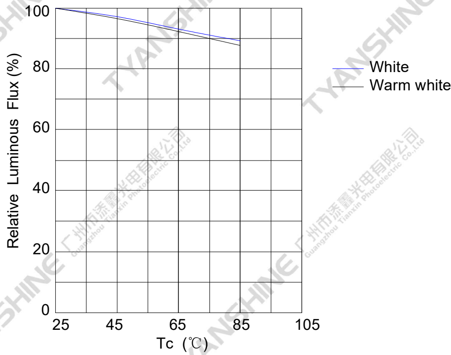
Temperature VS. Relative Luminous Flux (IF=500mA)
