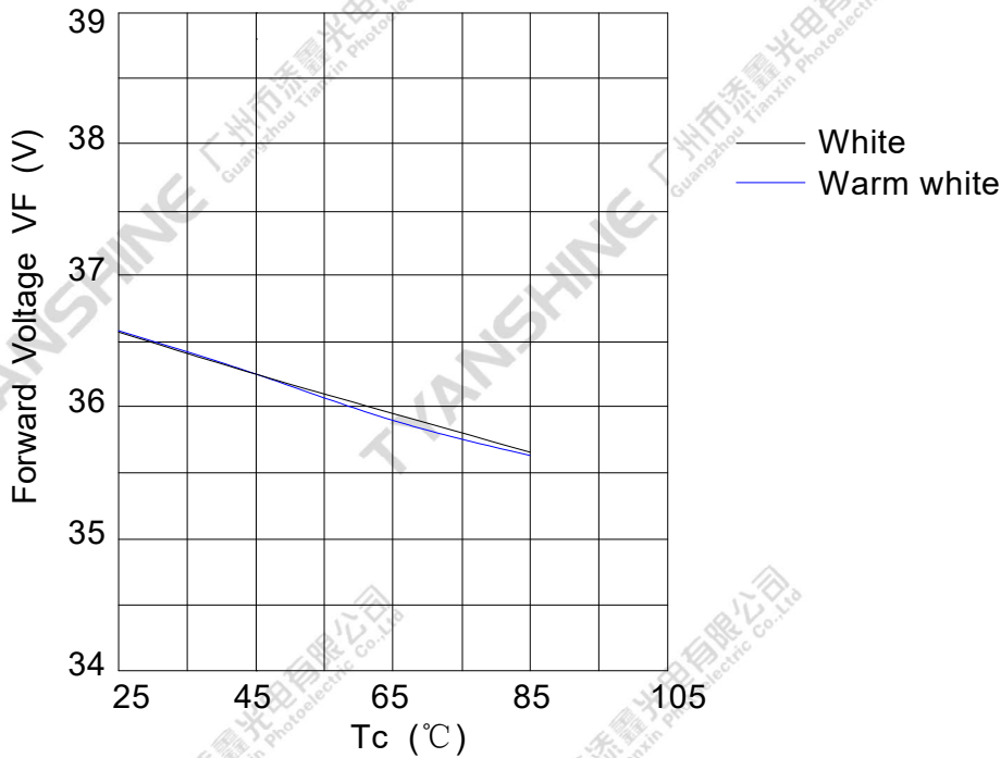
Temperature VS. Forward Voltage (IF=500mA)
